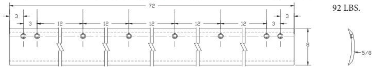
GRADER EDGE #GB20343 - 5/8" HOLES - 5/8" x 8" x 84" CDB - (9) SQ. CTSK. HOLES
