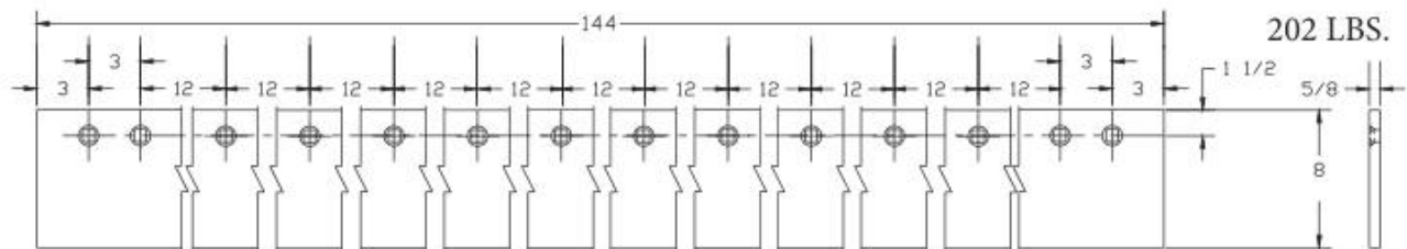
CARBIDE INSERTED PLOW BLADE #CB15082 - 5/8" HOLES - 3/4" x 6" x 35 15/16" FSE - (5) SQ. CTSK. HOLES
