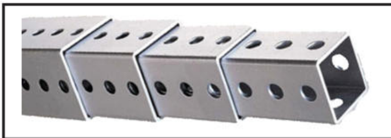
Part No. NS134SQ 1 3/4" Square Post Anchor
