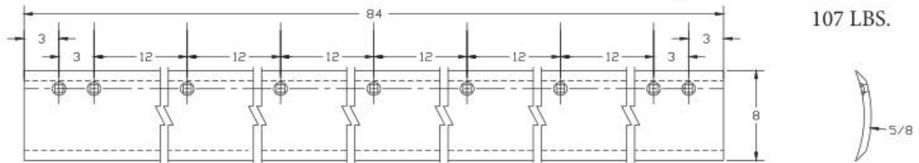
GRADER EDGE #GB20367 - 5/8" HOLES - 5/8" x 8" x 96" CDB - (10) SQ. CTSK. HOLES
