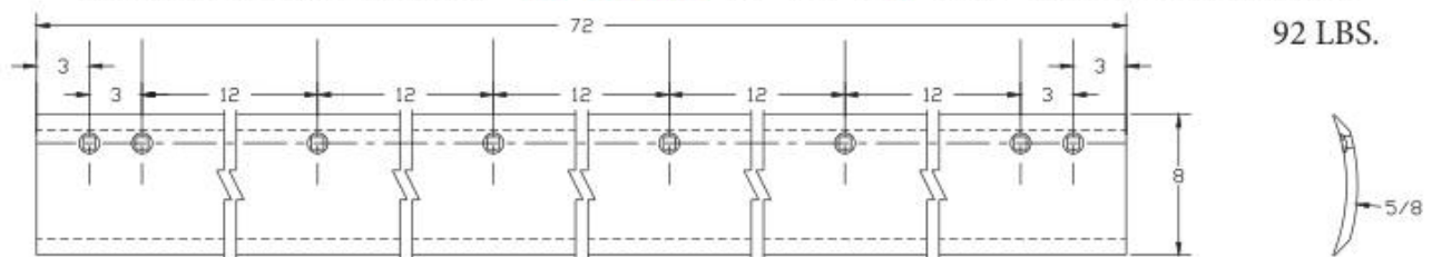
GRADER EDGE #GB20355 - 3/4" HOLES - 5/8" x 8" x 84" CDB - (9) SQ. CTSK. HOLES
