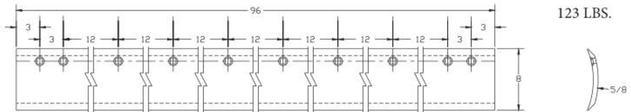
GRADER EDGE #GB20331 - 3/4" HOLES - 5/8" x 8" x 72" CDB - (8) SQ. CTSK. HOLES
