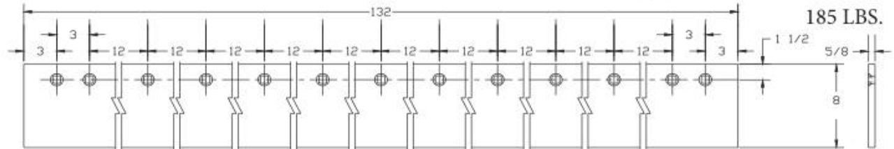
PLOW BLADE #BB20321 - 5/8" HOLES - 5/8" x 8" x 144" FSE - (14) SQ. CTSK. HOLES
