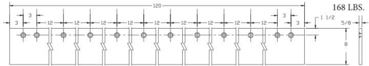
PLOW BLADE #BB20315 - 5/8" HOLES - 5/8" x 8" x 132" FSE - (13) SQ. CTSK. HOLES
